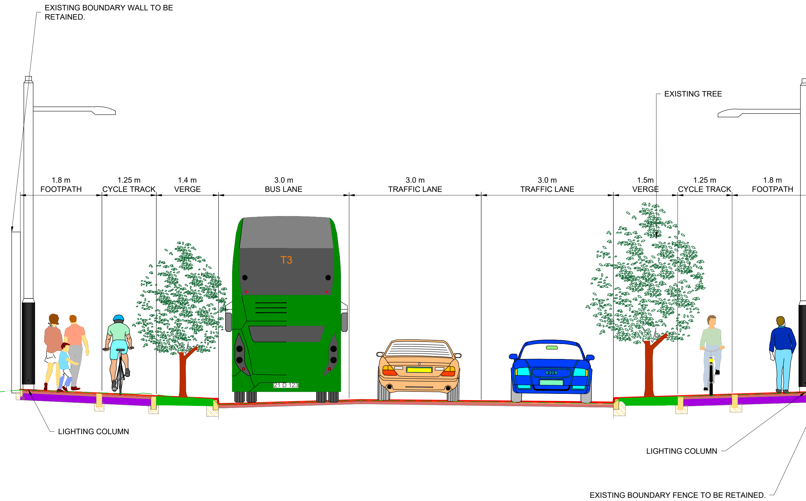
TYPICAL SECTION E-E ST. MOBHI ROAD LOCATED ON GA SHEET 08 DRAWING REF: BCIDD-ROT-GEO_GA-0304_XX_00-DR-CR-0008
