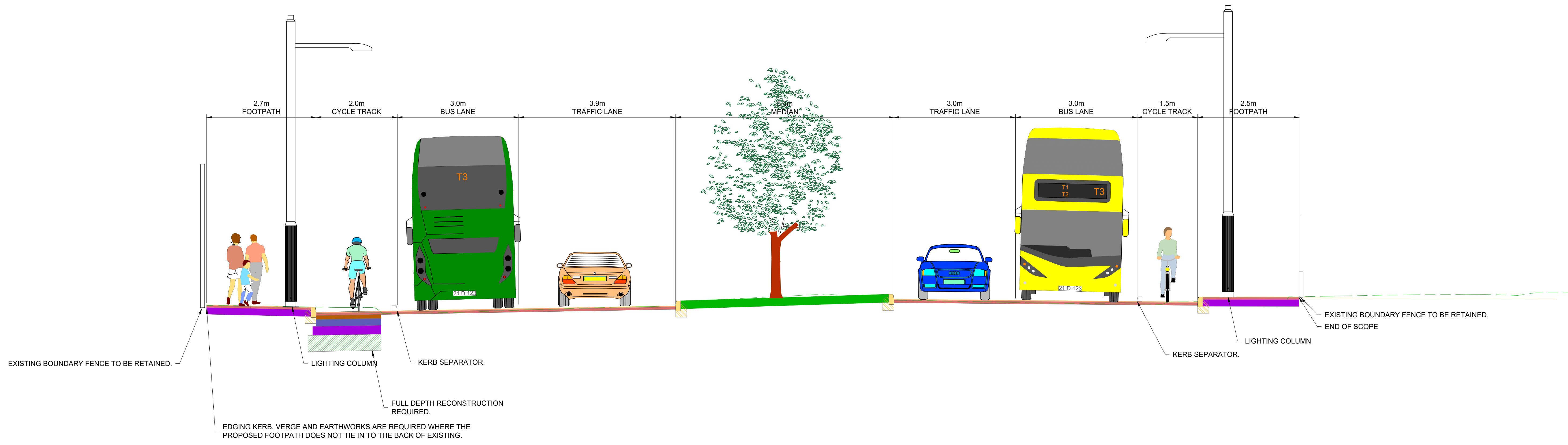
TYPICAL SECTION R-R FINGLAS ROAD
